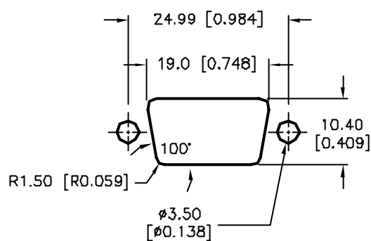
Panel Cutout
