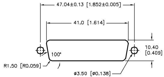
Panel Cutout
