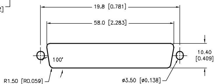
Panel Cutout
