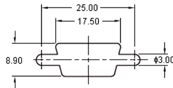
Panel Cutout
