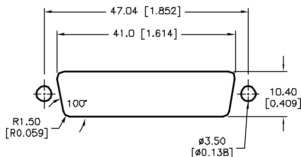
Panel Cutout
