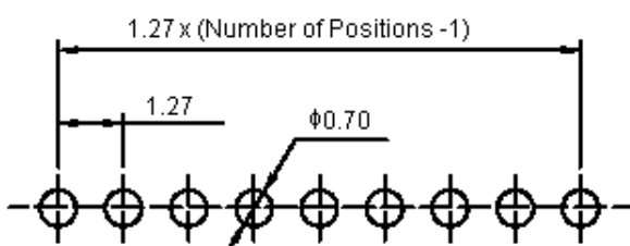
PCB Layout
