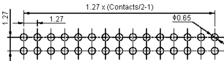
PCB Layout
