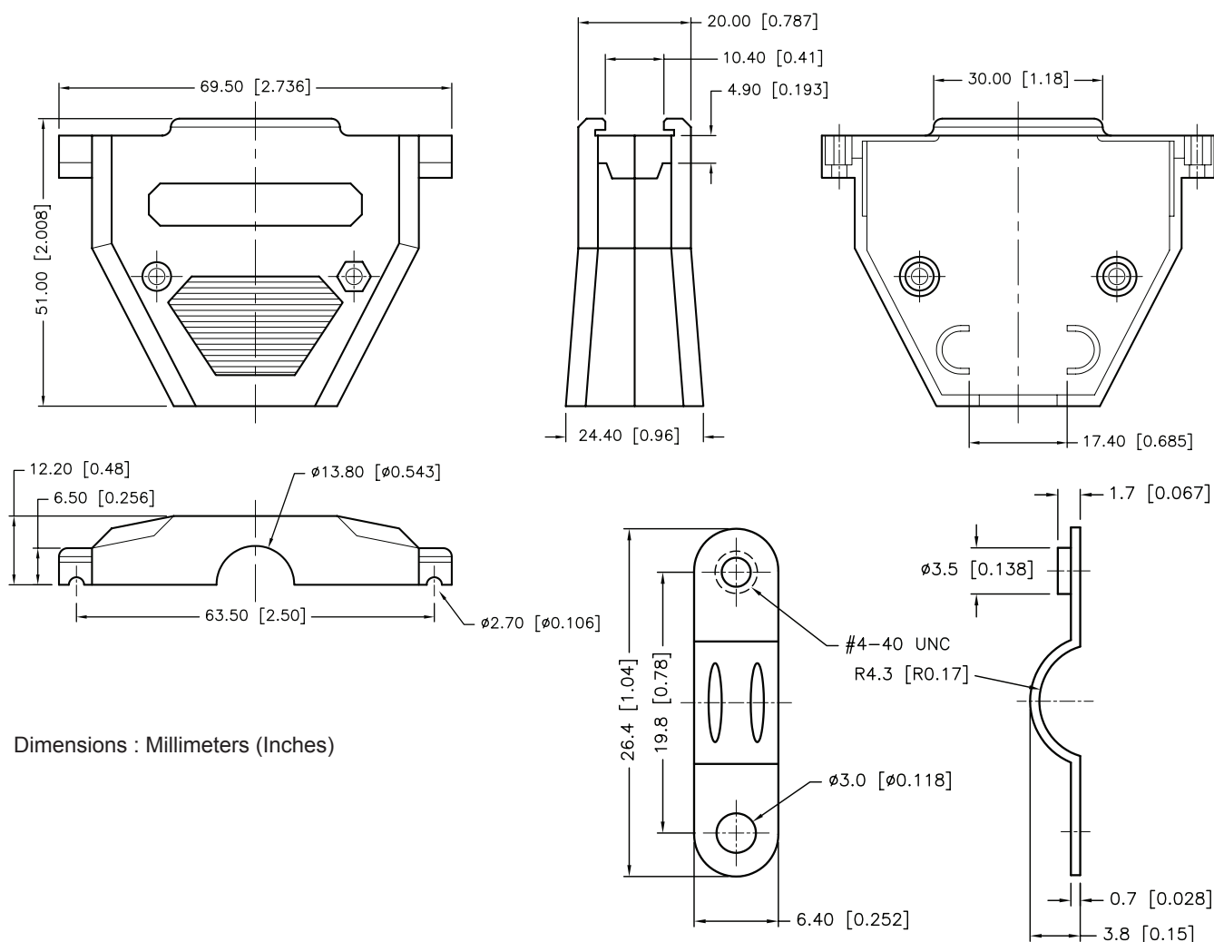
Cable Clamp (2Pcs)
