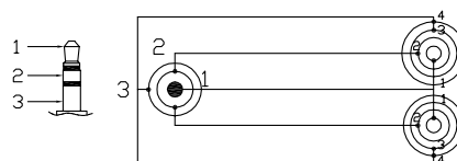
Soldered Drawing: 3.5mm Stereo Plug 2×3.5mm 4 Pole Jacks
