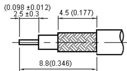
Stripping Dimension
