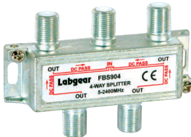
FBS904 Broadband 4 way compact splitter, power pass all ports
