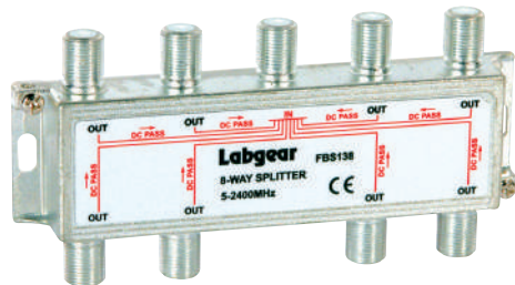
FBS138 Broadband 8 way compact splitter, power pass all ports
